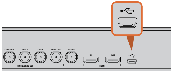
HyperDeck Studio USB port
