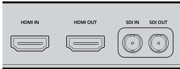
HyperDeck Shuttle HDMI and SDI outputs.
