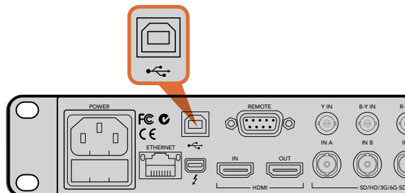
HyperDeck Studio Pro USB port
