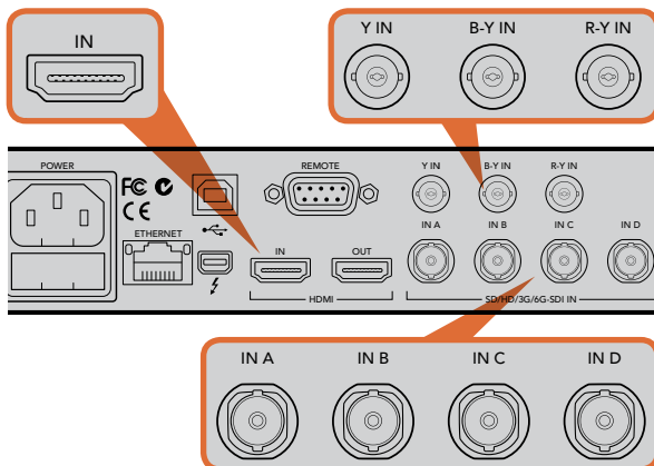
HyperDeck Studio Pro HDMI, analog component and SDI inputs.
