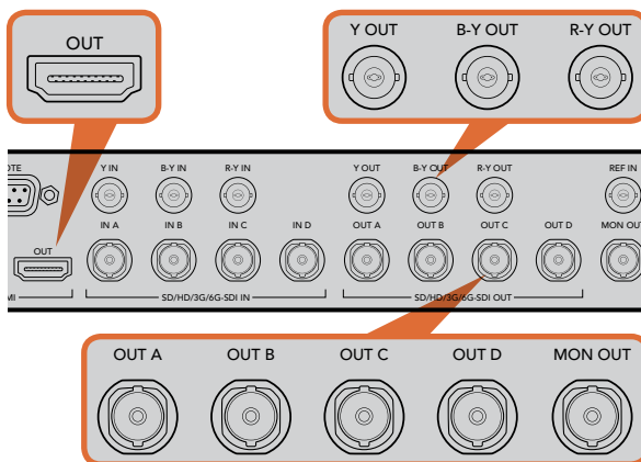
HyperDeck Studio Pro HDMI, analog component and SDI outputs plus Monitor Out.
