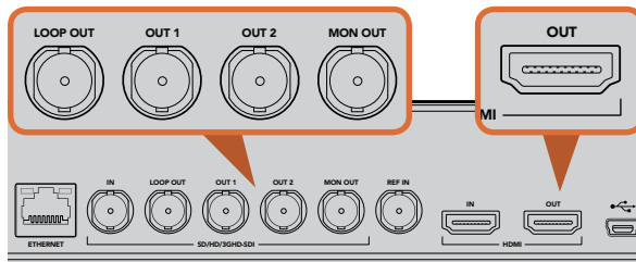
HyperDeck Studio SDI and HDMI outputs. SDI outputs include a Loop Out and a Monitor output.
