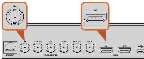
HyperDeck Studio SDI and HDMI inputs
