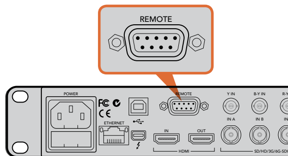
Remote port on HyperDeck Studio Pro
